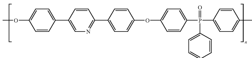
Polymer 1
